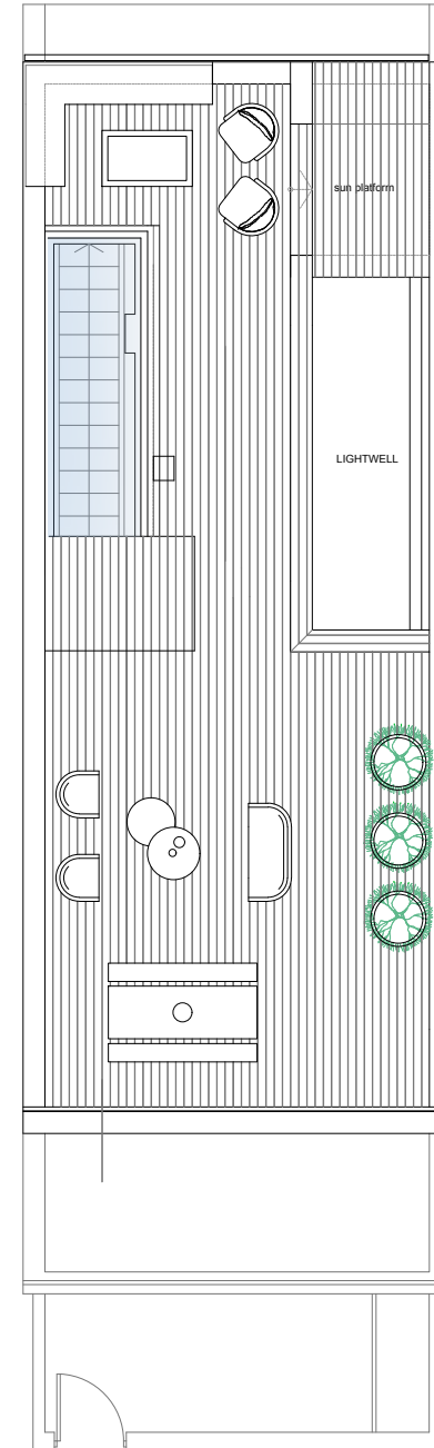
ROOF PLAN
